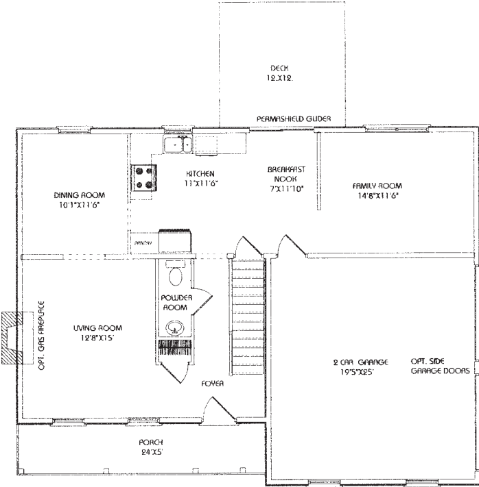
1st floor
